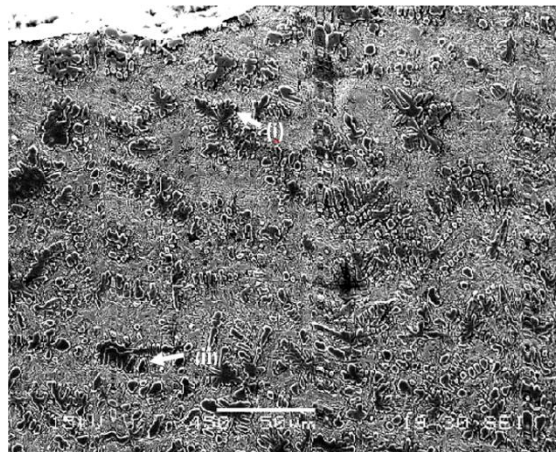
Figure 6. location near the arc source showing many reprecipitation of TiC structures with (i) of a flower type of TiC and (ii) globular.
